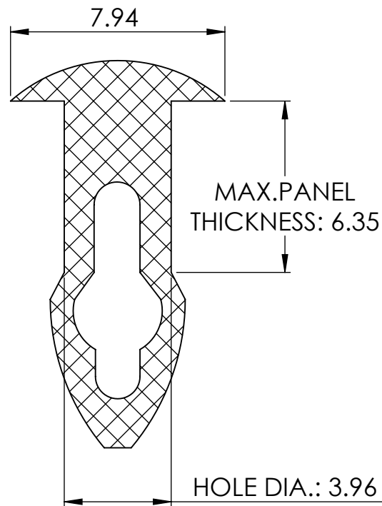
SECTION Y-Y
